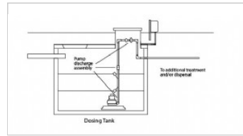
Dosing tank discharge assembly
