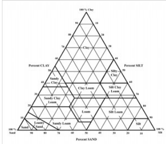
Soil textural classes - USDA
