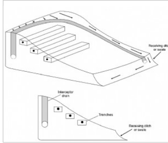
Drain, interceptor
