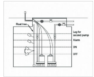
Demand dosing, duplex pumps and float controls
