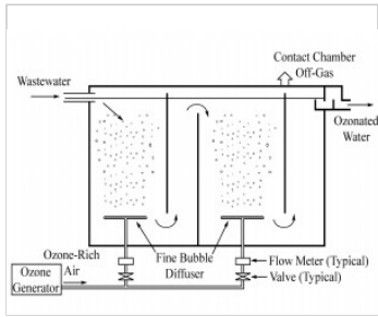
Ozone generator
