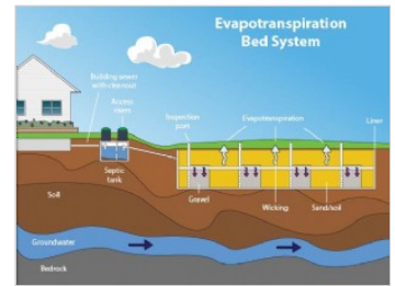
Evapotranspiration bed
