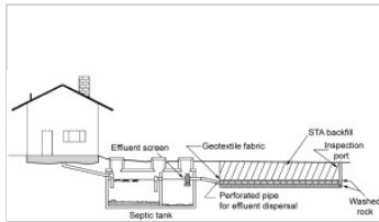
Gravity distribution sytem, profile
