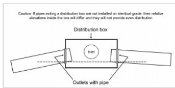
Distribution box with inlet and outlets
