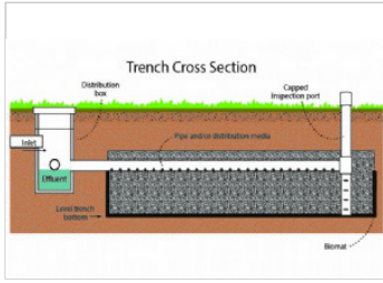
Conventional trench detail profile view
