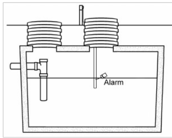
Holding tank with the water level in alarm status
