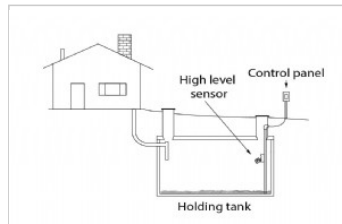
Holding tank connected to house
