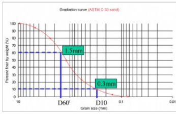
Gradation curve for ASTM C-33 sand
