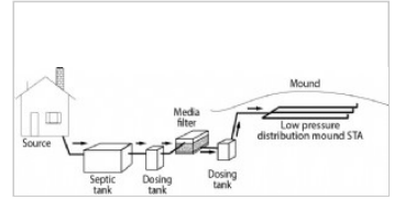
Example OWTS ST, SP media filter, LPD distribution
