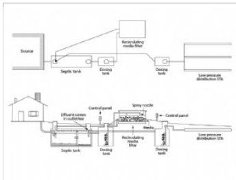
Recirculating media filter to low pressure distribution STA
