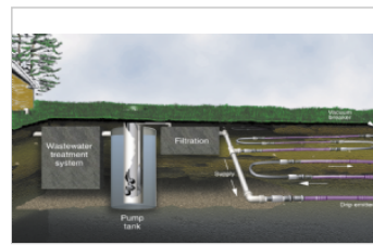
Drip distribution STA
