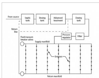
Drip distribution generic treatment train
