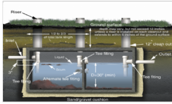
Septic tank diagram
