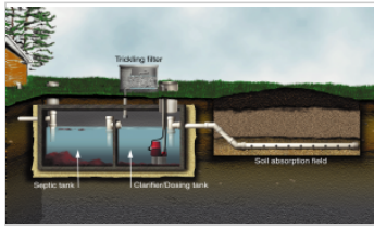
Recirculation trickling filter with trench distribution STA
