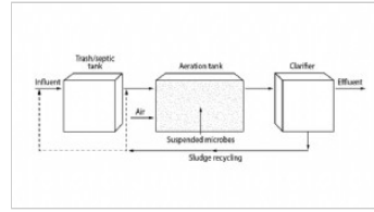
Generic suspended growth treatment process Trash/septic tank, generic ATU using suspended growth treatment process, profile view
