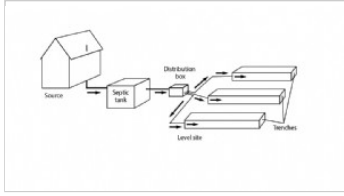
Gravity parallel trenches
