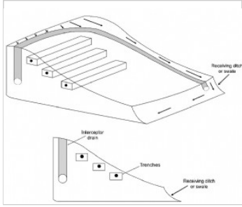
Drain, interceptor
