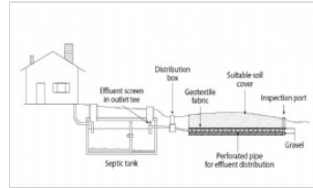
Gravity distribution system
