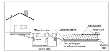
Gravity distribution system, profile
