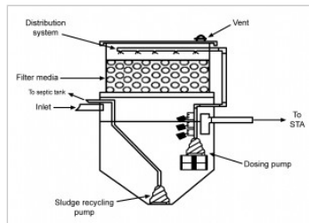
Trickling filter schematic, profile
