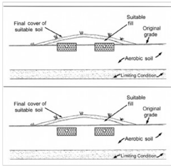
Final cover backfill over an STA
