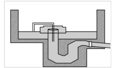
Effluent exiting the pump tank through the dosing siphon part 2
