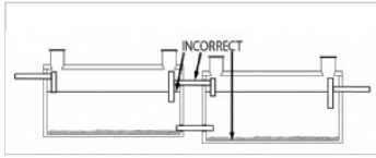
Septic tank multiple tank overflow baffle incorrect drop elevation with sludge pipe configuration
