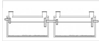
Septic tank multiple tank overflow baffle same elevation configuration
