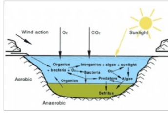
Treatment processes in facultative lagoons
