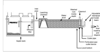
Example constructed wetland treatment train
