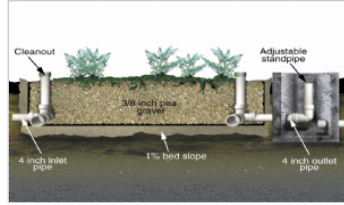
Constructed wetland treatment unit
