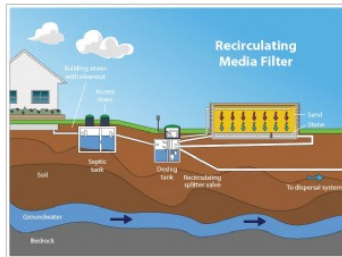
Recirculating media filter, split base Residential OWTs: gravity septic tank, dosing tank, recirculating media filter with split base, recirculating splitter valve, profile view, color
