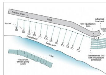
Lakefront STEP cluster system to LPD
