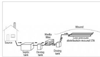
Example OWTS ST, SP media filter, LPD distribution
