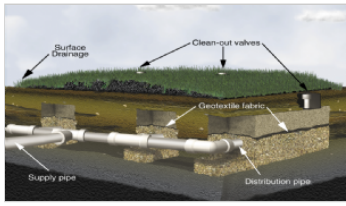
Low pressure distribution STA
