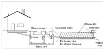
Gravity distribution sytem, profile
