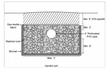
Conventional trench detail
