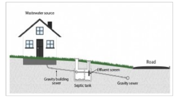
Building sewer series - House with STEG
