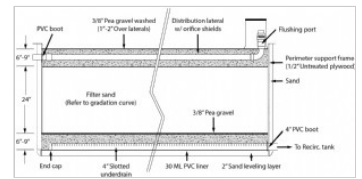
Recirculating sand filter detail
