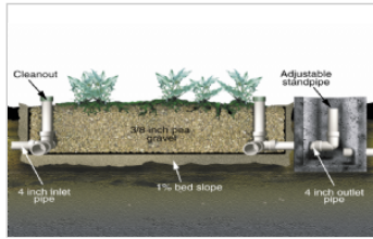
Constructed wetland treatment unit
