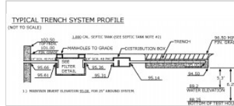
Example treatment train profile construction detail
