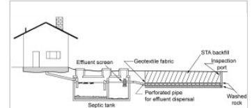
Gravity distribution system, profile
