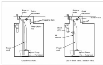
Discharge assemblies showing device options
