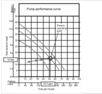
Pump selection based upon a system curve
