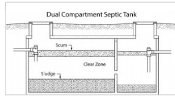
Dual compartment septic tank solids separation Two compartment septic tank showing baffle wall and solids separation, profile view
