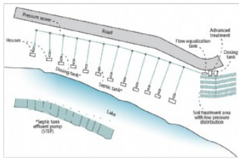
Lakefront STEP cluster system to LPD
