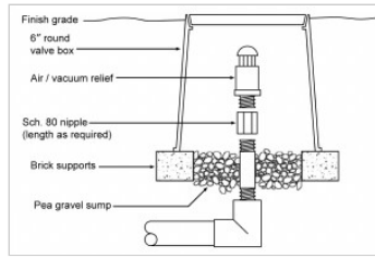
Configuration of an air release valve
