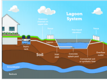
Lagoon system Residential OWTS: gravity septic tank, lagoon, profile view, color
