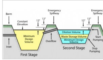
Two stage lagoon cross section Two stage lagoon with designations for design and storage requirements, cross section
