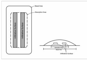
Absorption area level site
