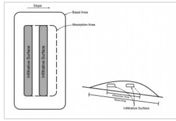
Absorption area sloping site
