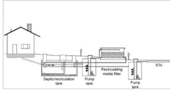
Config 1 for recirculating media filters, separate, profile
