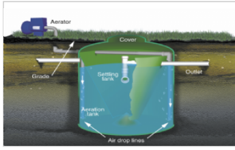
Aerobic treatment unit
