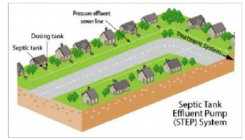
Community STEP system
