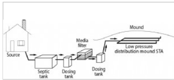
Example OWTS ST, SP media filter, LPD distribution
