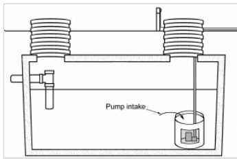
Dosing tank, pump basin, pump intake Dosing tank with pump installed in pump basin to raise intake above accumulating solids
