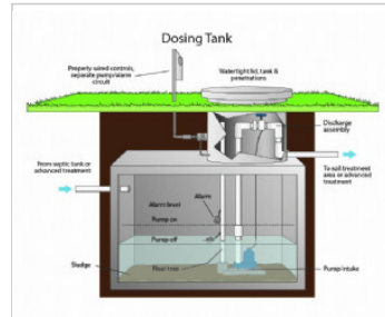
Dosing tank, block, pump demand dosing Dosing tank with the pump installed on a block, demand dosed float configuration, profile view, color
