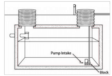
Dosing tank, pump on block, pump intake Dosing tank with pump installed on block to raise intake above accumulating solids
