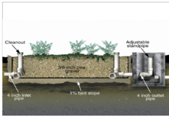
Constructed wetland treatment unit
