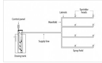
Spray distribution system generic treatment train
