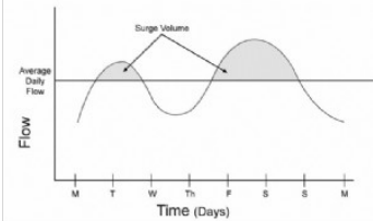
Volume, surge
