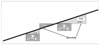
Benching for trench construction
