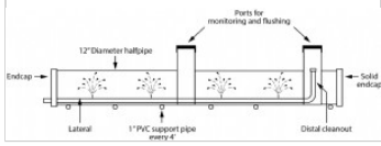
Shallow narrow trench detail
