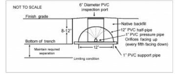
Shallow narrow trench cross section
