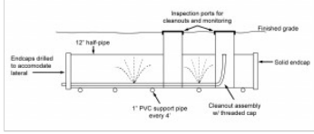
Shallow narrow trench profile
