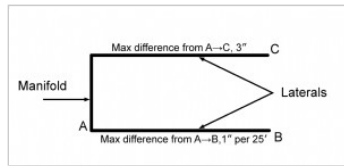
Elevation difference across a level STA
