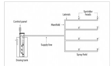
Spray distribution system generic treatment train Dosing tank, spray distribution STA, profile view
