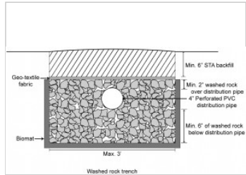
Washed rock trench cross section
