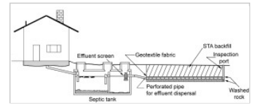
Gravity distribution sytem, profile
